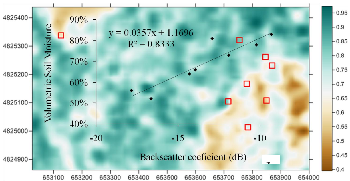
Fig. 2. The estimation map for moisture content in a large area of Goshikigahara created using the linear model which uses the correlation between the microwave backscattering coefficient (dB) and the surveyed VSM data (at measurement points shown as mark (□)). 0.4 (40%)-0.95 (95) in the legend is the soil moisture content.
