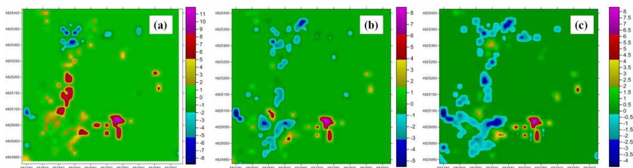
Fig. 3. Differences in backscattering coefficients ( \Delta\sigma_{dB}^0 ) of dwarf bamboo distribution area in the Goshikigahara area on Taisetsu Mountains (Where, (a) shows the difference backscattering coefficients ( \Delta\sigma_{dB}^0 ) between July 6 and June 19, 2010; (b) shows the difference backscattering coefficients ( \Delta\sigma_{dB}^0 ) between August 21 and August 4, 2010; and (c) shows the difference backscattering coefficients ( \Delta\sigma_{dB}^0 ) between October 6 and September 19, 2010).
