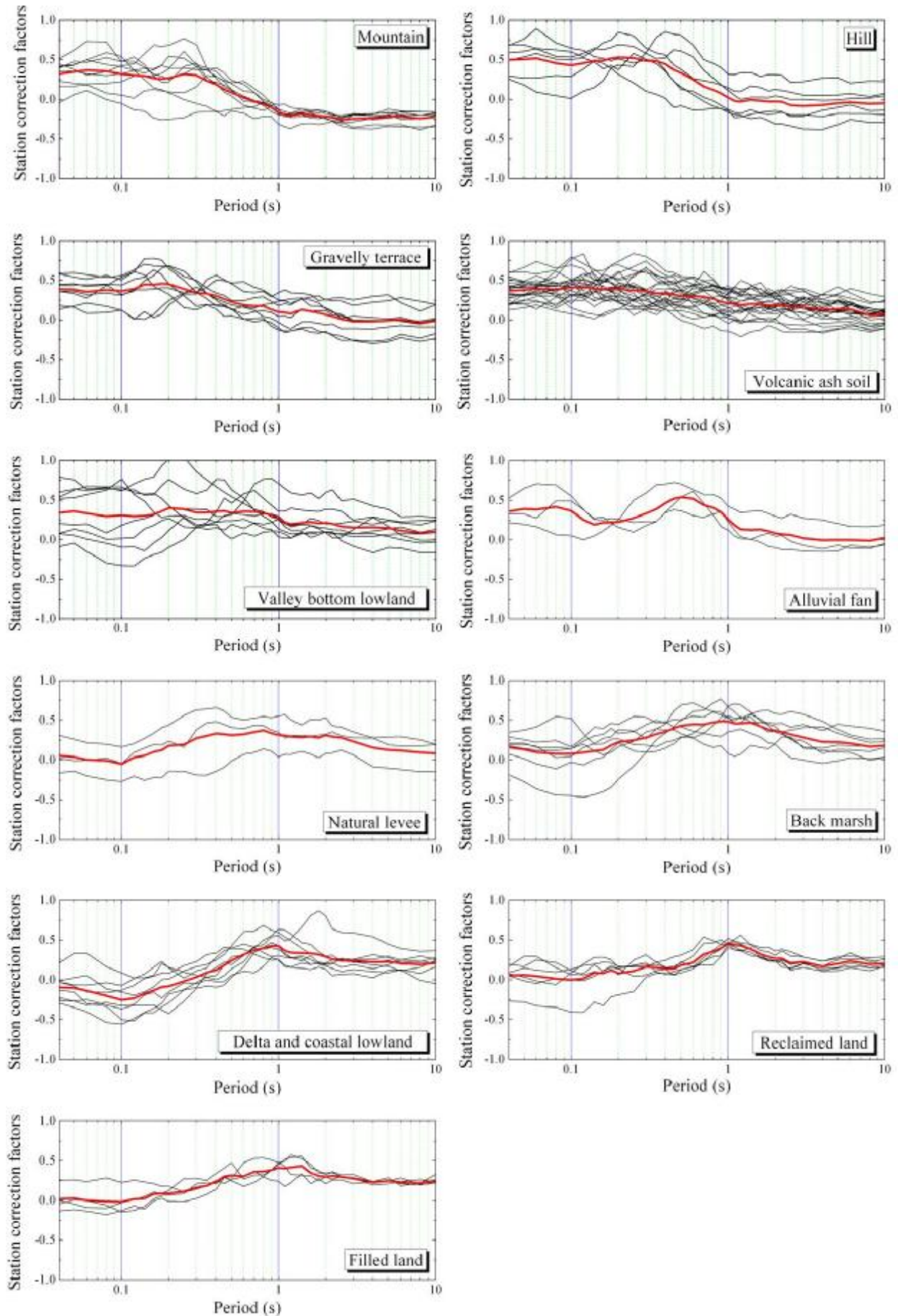
Figure 7: The station correction factors with respect to the geomorphologic classifications. The red line shows the average of the station correction factors.
