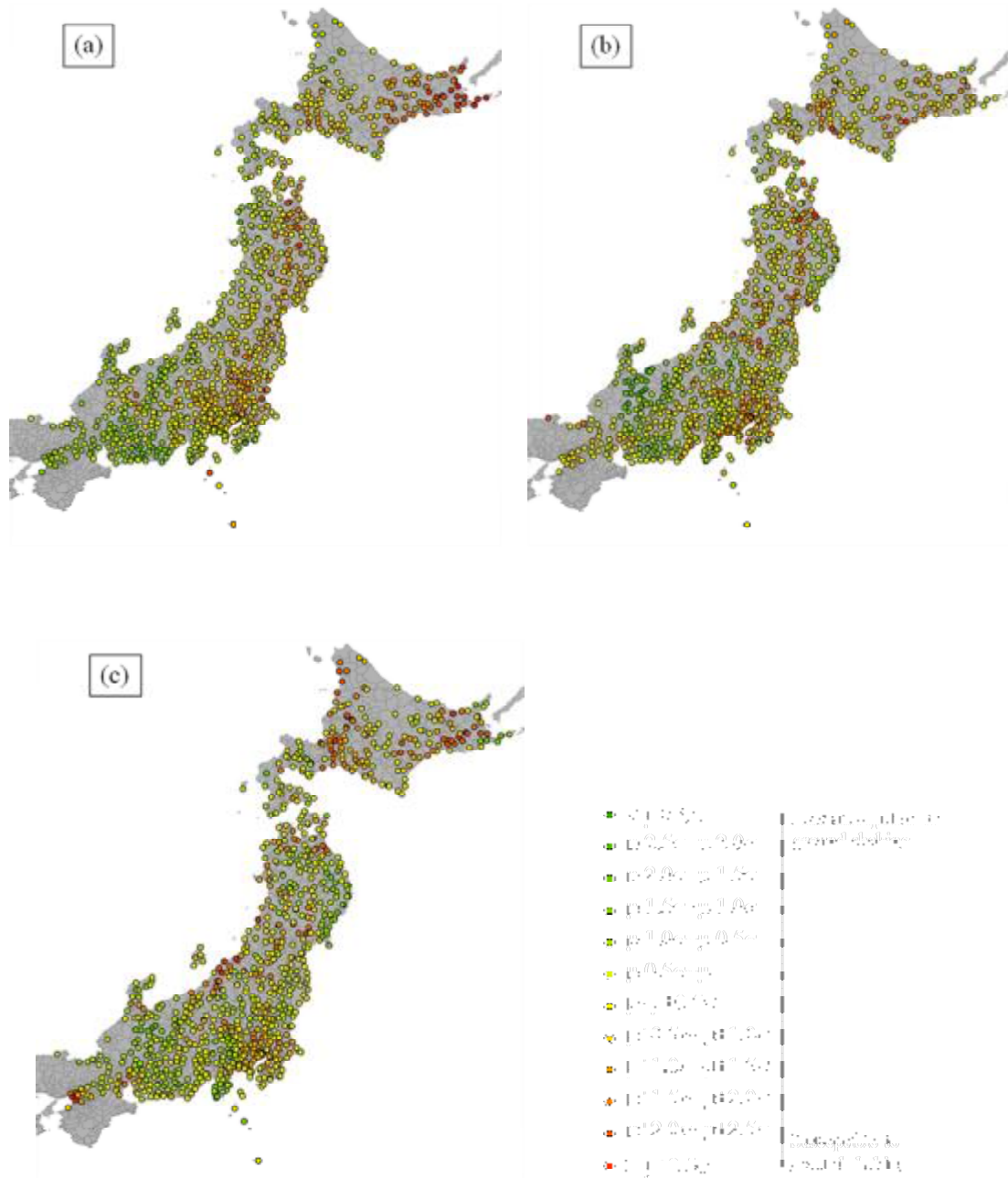
Figure 5: Illustration of station correction factors for the period of (a) 0.2 s, (b) 1.0 s, and (c) 5.0 s.
