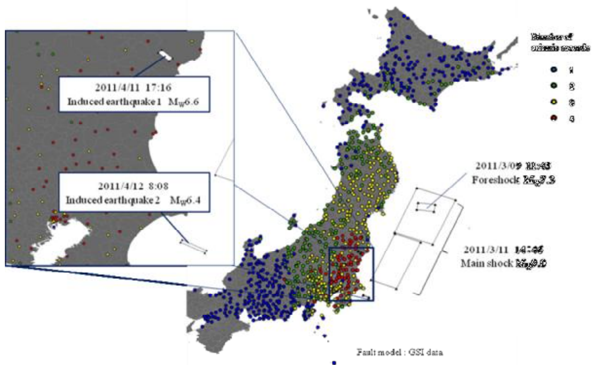
Figure 1: Earthquake source faults and the seismic observation stations used in this study.
