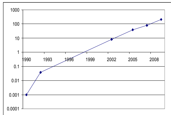
Fig.3 data rates (Mbps) of SSTL satellites 1990-2010
