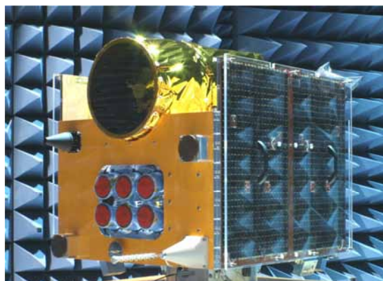
Fig.9 Beijing-1 enhanced DMC microsatellite 2005
