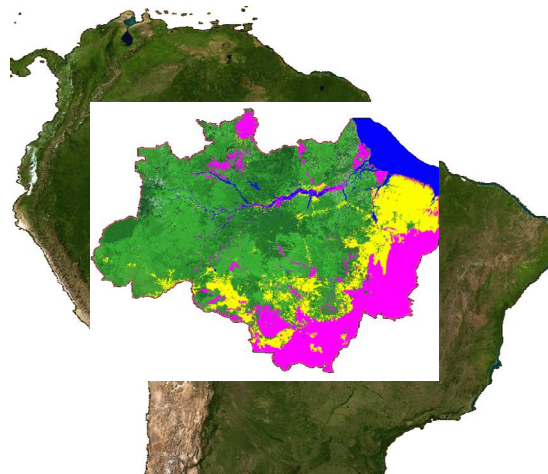
Fig.18 'Land cover/Forest map of Brazilian Amazon basin (© INPE)
