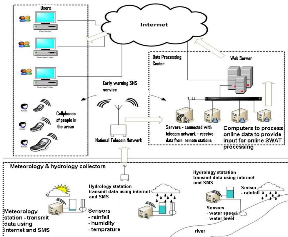
Figure 4. The general methodology for the online supporting system flood warning in Vu Gia watershed, Quang Nam province, Vietnam
