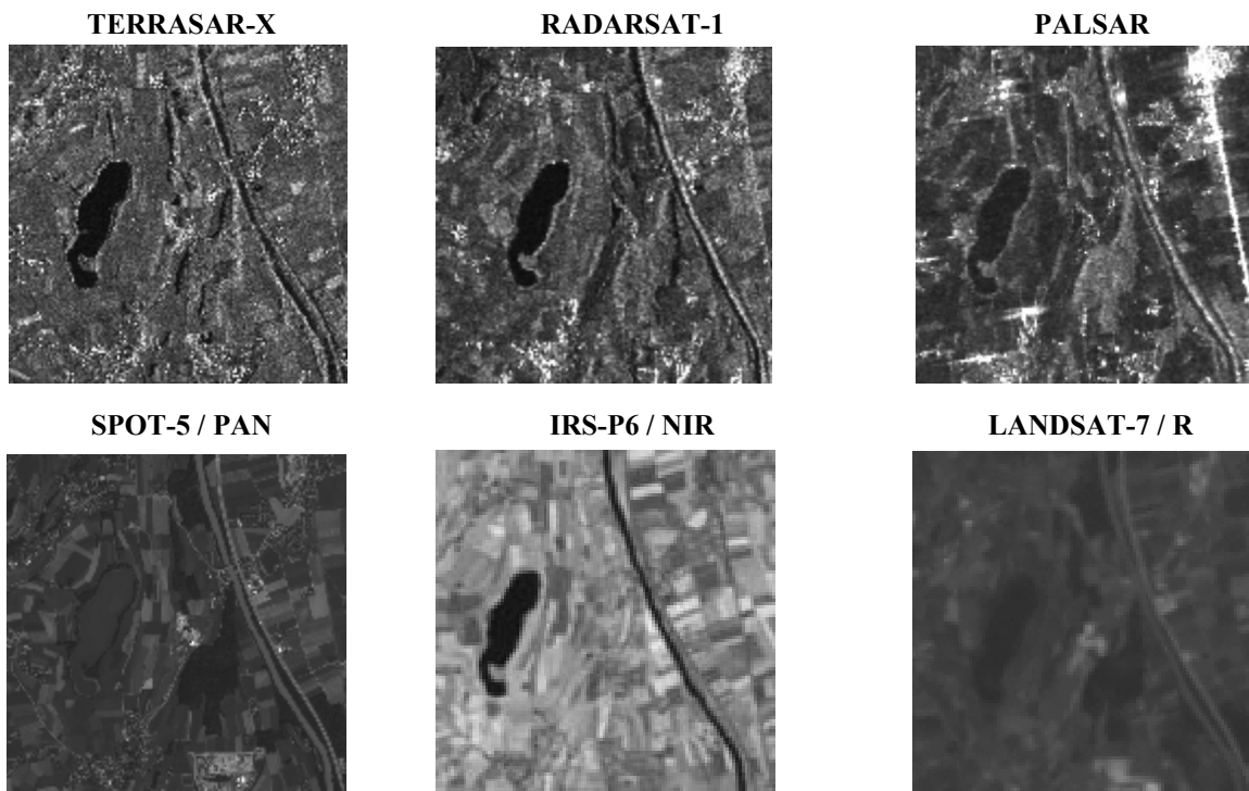
Figure 2: Examples of image parts from the different sensor data to be matched. Notice the huge differences not only between SAR and optical images (top to bottom), but also between SAR and between optical images.
