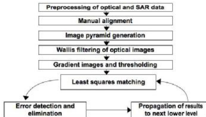
Figure 3: Overview of processing steps.
