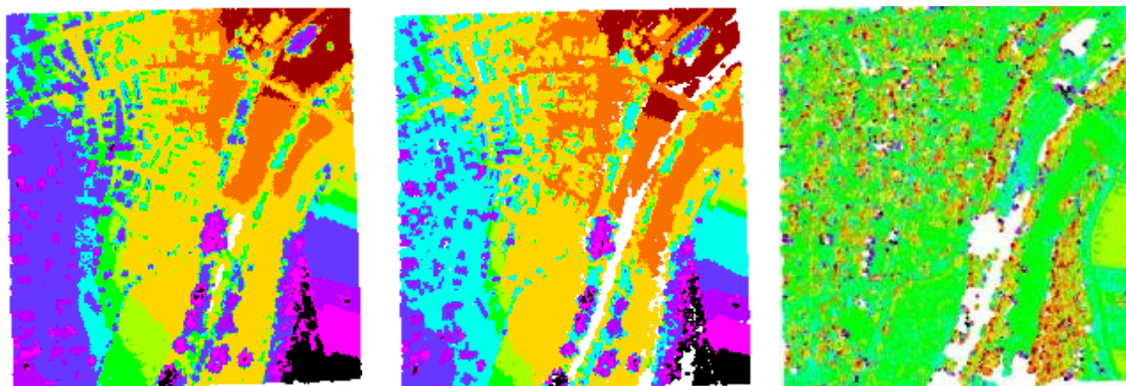
Figure 6: Colour-coded differences of matching DSM to reference ALS DSM. Left: No error detection ; Middle: Cross-correlation < 0.6 ; Right: Test no. 2 above. Greenish colours represent the smallest errors, white non-matched/rejected match-points. Note: although in the 3 figures the same numbers of intervals are used, their range varies, especially for the right figure, where the range of each colour is smaller.
