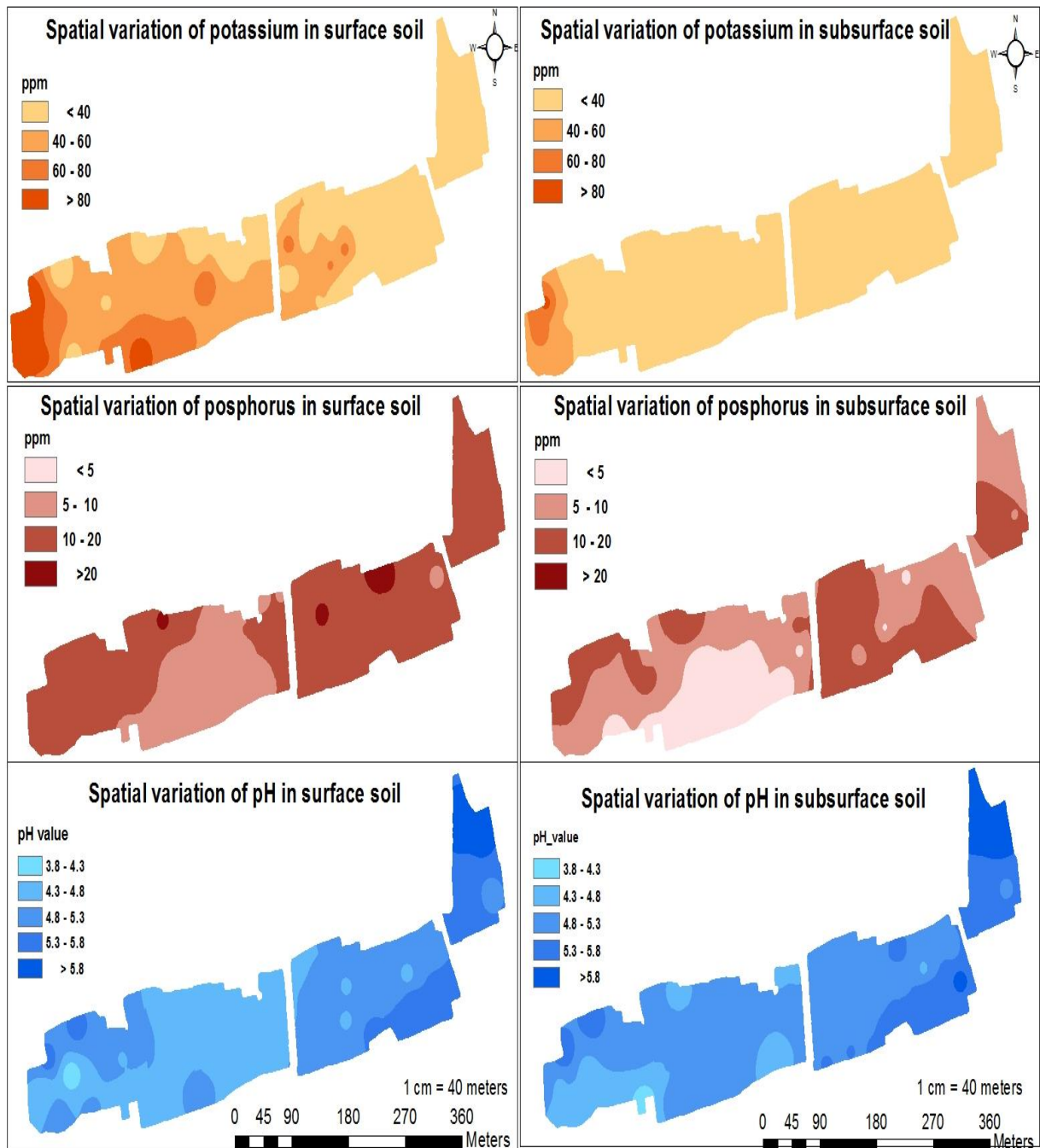
Figure 4. Spatial variation of pH, K and P in surface and sub-surface soils in the area
