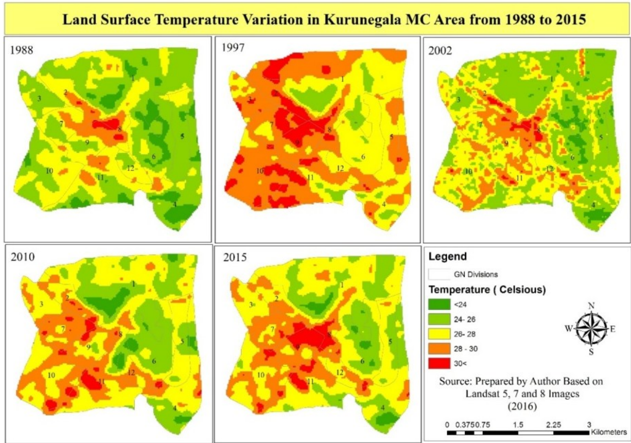
Figure 2: LST Variation in Kurunegala MC from 1988 to 2015
