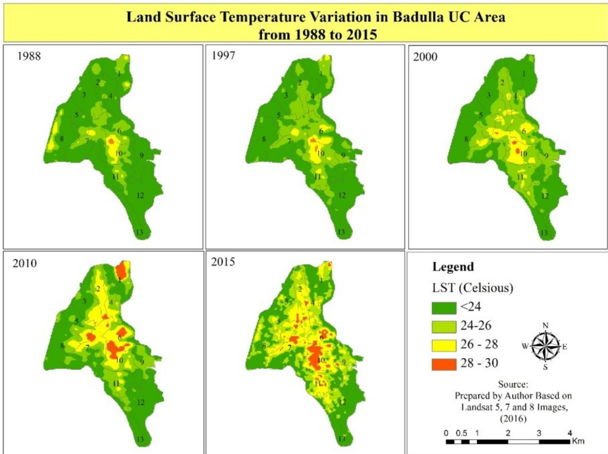
Figure 3: LST Variation in Badulla MC from 1988 to 2015
