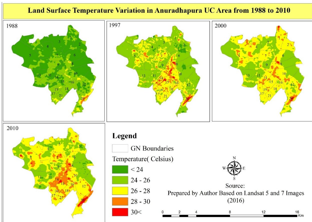
Figure 5: LST Variation in Anuradhapura MC from 1988 to 2010
