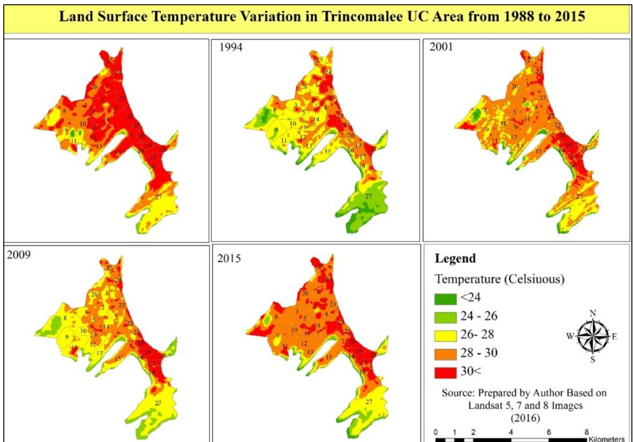
Figure 7: LST Variation in Trincomalee UC from 1988 to 2015
