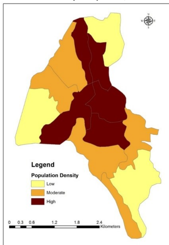
Figure 4: Population Density of Badulla MC in 2012
