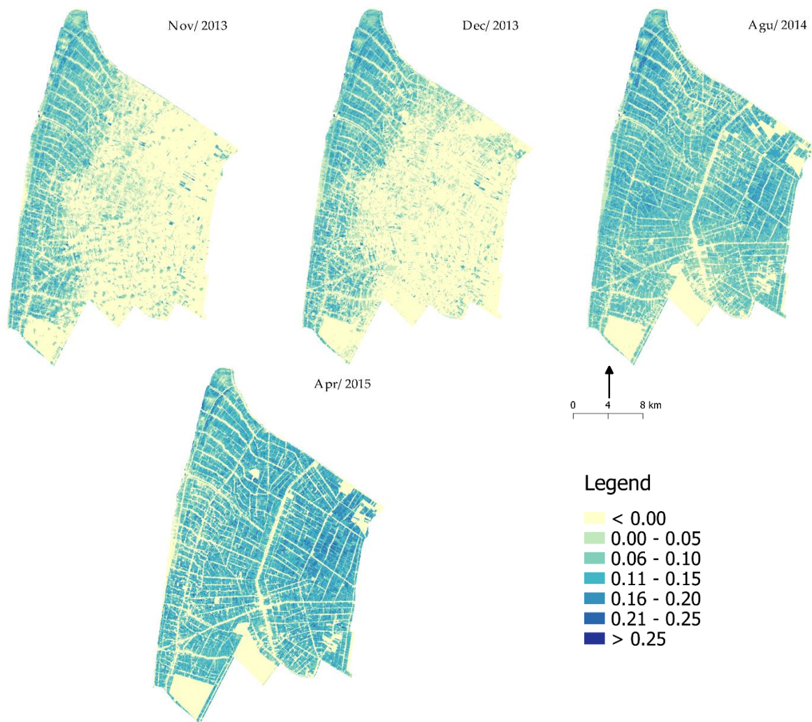
Fig 6. Threshold value of MNDWI maps on Landsat 8 imagery in An Minh district
