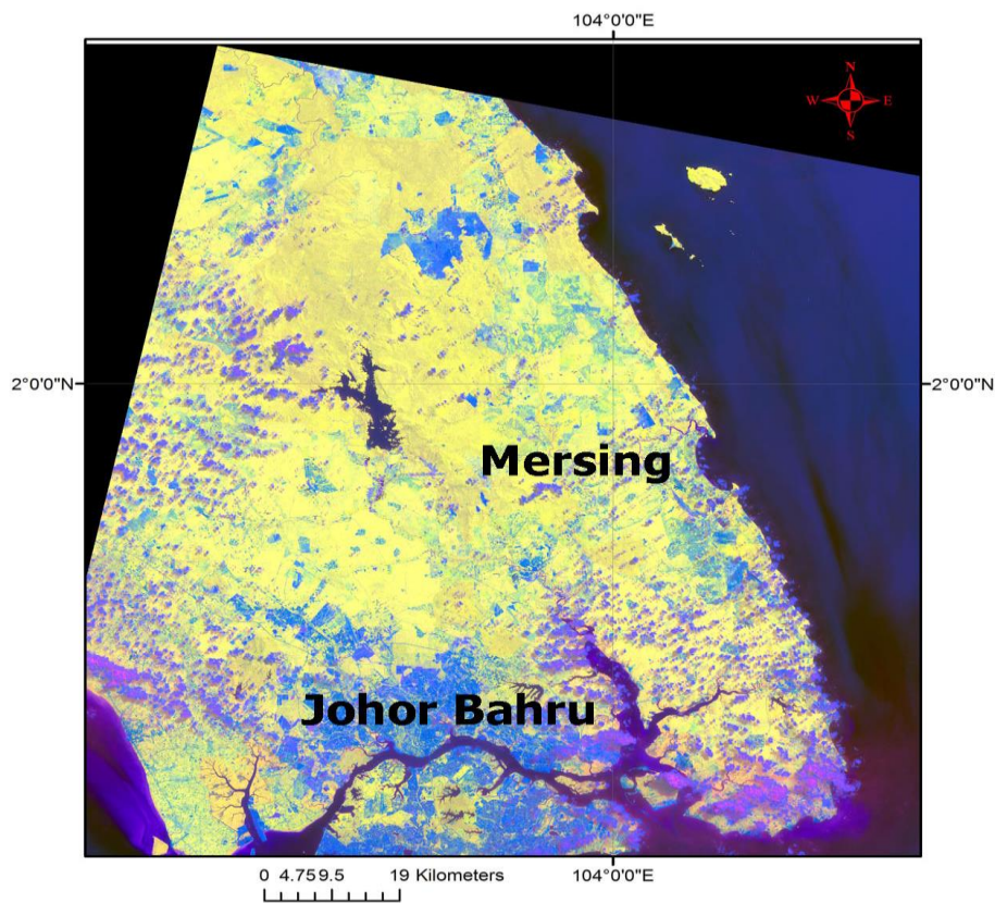
Figure 2. RGB colour combination of band ratio of 5/7, 5/4 and 4/3 for Johor state.
