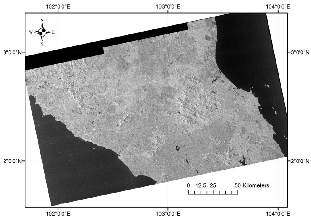
Figure 3. VH polarization channel of Sentinel-1 SAR scene covering Johor state.
