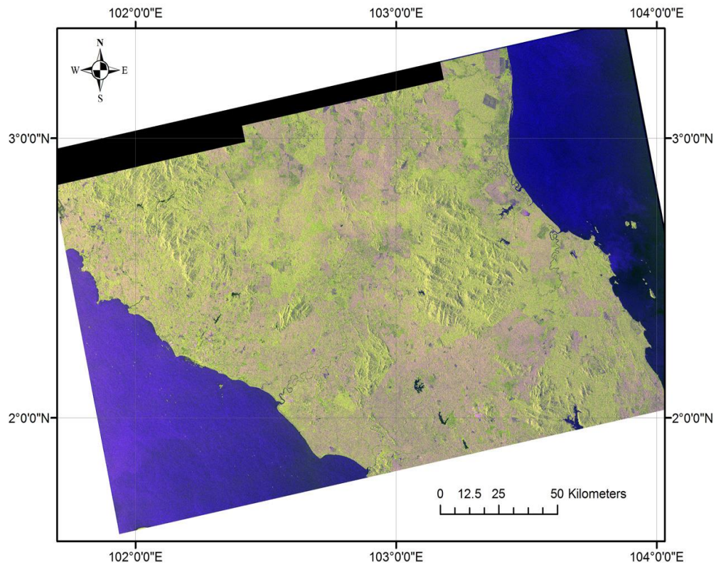
Figure 3. RGB colour combination (VH, VV and VH+VV polarization channels) of Sentinel-1 SAR scene covering Johor state.
