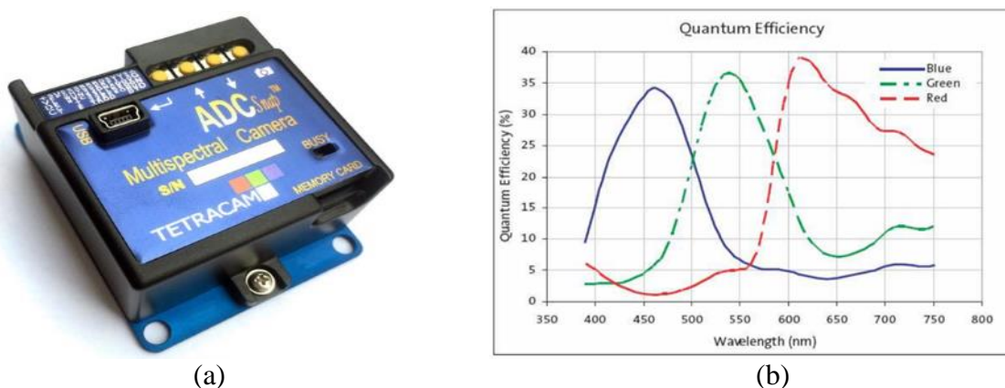
Figure 1. (a) ADC Micro multispectral camera (Tetracam, Inc., CA, USA) and (b) spectral response characteristics of the camera for blue that is blocked for NIR sensing, green, and red, employed in this study ( www.tetracam.com ).
