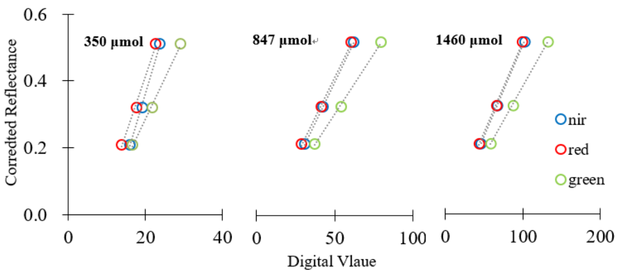
Figure 4. Relationships between corrected reflectance and estimated tarp digital values for the wavebands of green, red, and near infrared (NIR).
