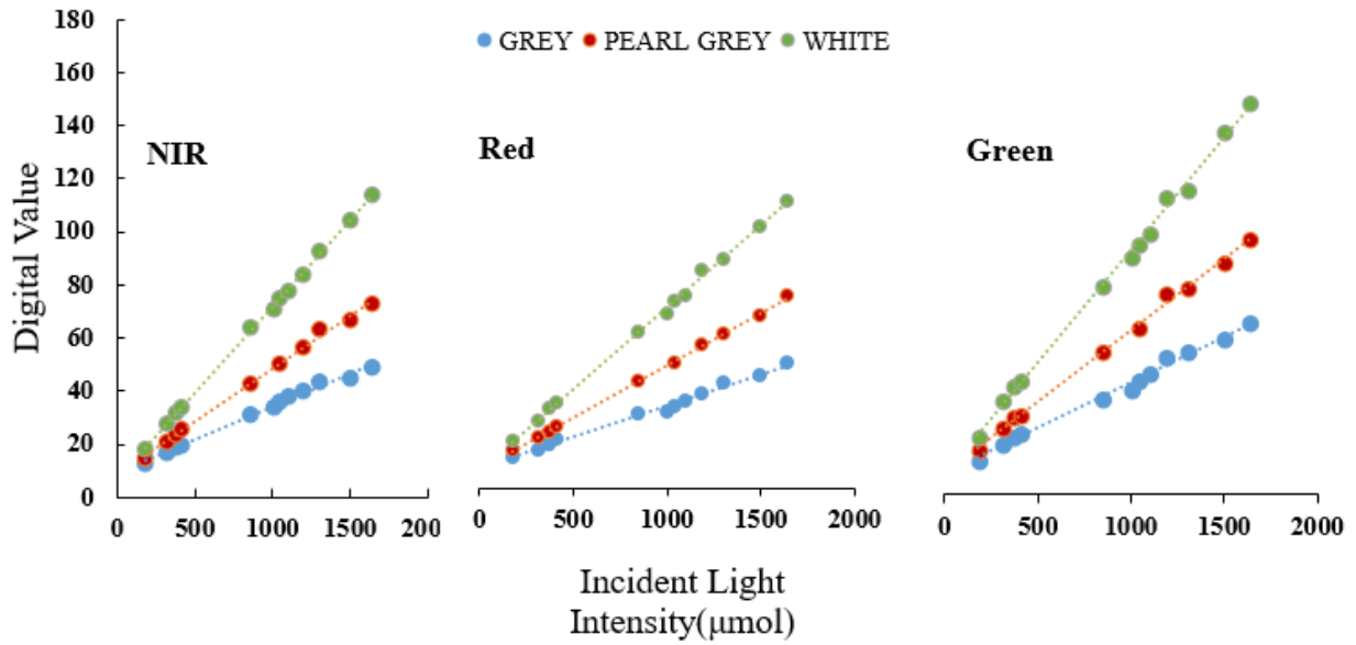
Figure 3. Relationships between DN values and incident light intensity of three reference tarps (grey, pearl grey, and white) for the wavebands of green, red, and near infrared (NIR).
