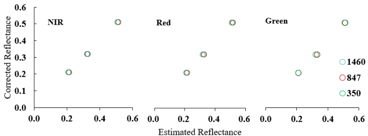
Figure 5. Comparisons between corrected reflectance using the UAV-based image calibration method and estimated reflectance of the three reference tarps at the light intensity values of 350, 847 and 1,460 \mu\text{mol} in UAV images for the wavebands of green, red, and NIR.
