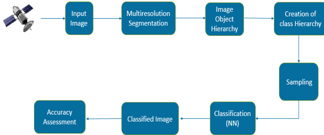
Figure 1. A framework for non-linear object classification using the OBIC
