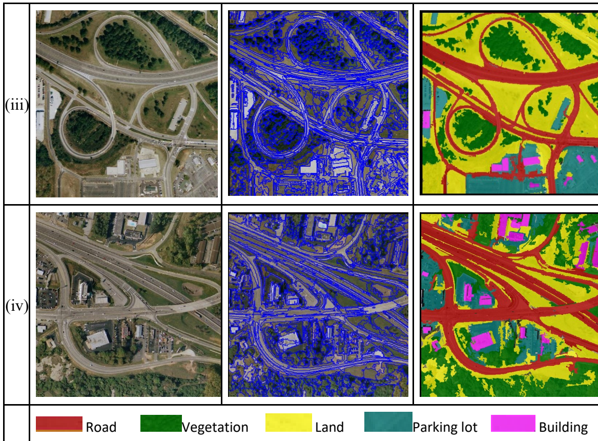
Figure 4. Developed Suburban images: (a) input image, (b) segmented images, (c) classified images in road, vegetation, land, parking lot area and building objects.
